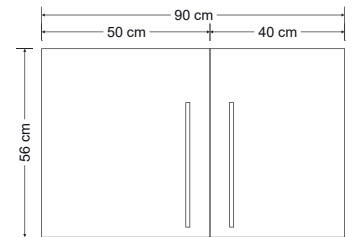
HS 90 - drawing
