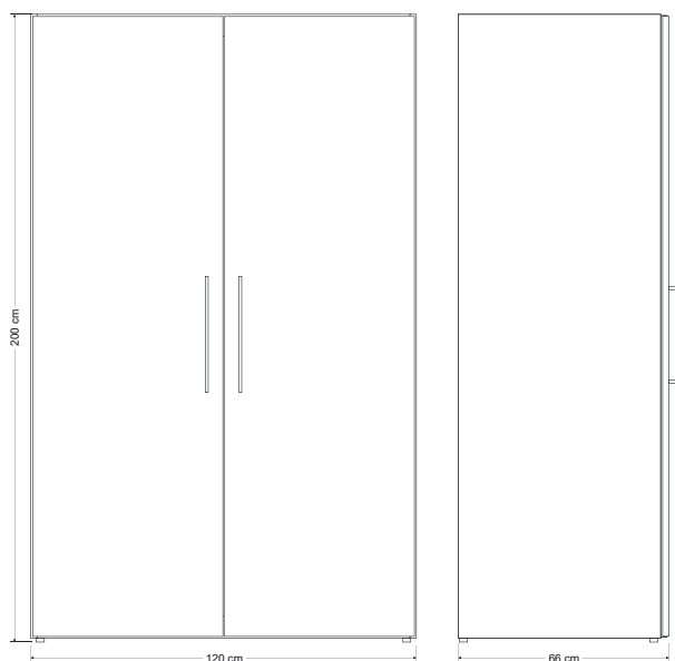
drawing: SKM 120 - measures
